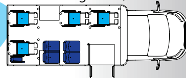
4+2 Passenger 4 w/c
