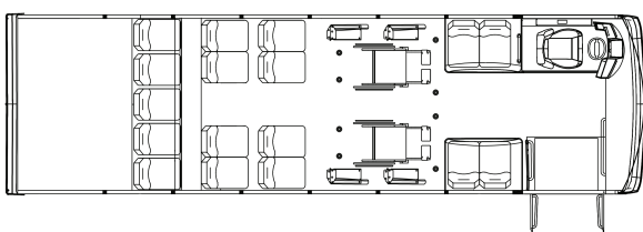
35', 24 Passengers, 2 w/c
