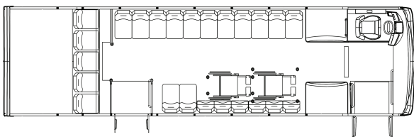
35', 24 Passengers, 2 w/c
