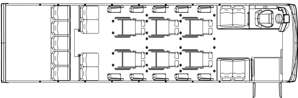
35', 33 Passengers, 6 w/c
