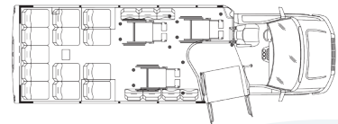
26', 13+7 Passenger, 3 w/c
