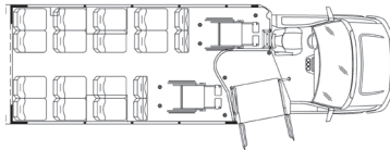
26', 14+4 Passenger, 2 w/c
